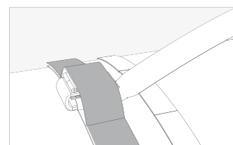
6 - Everything is set under the top webbing
